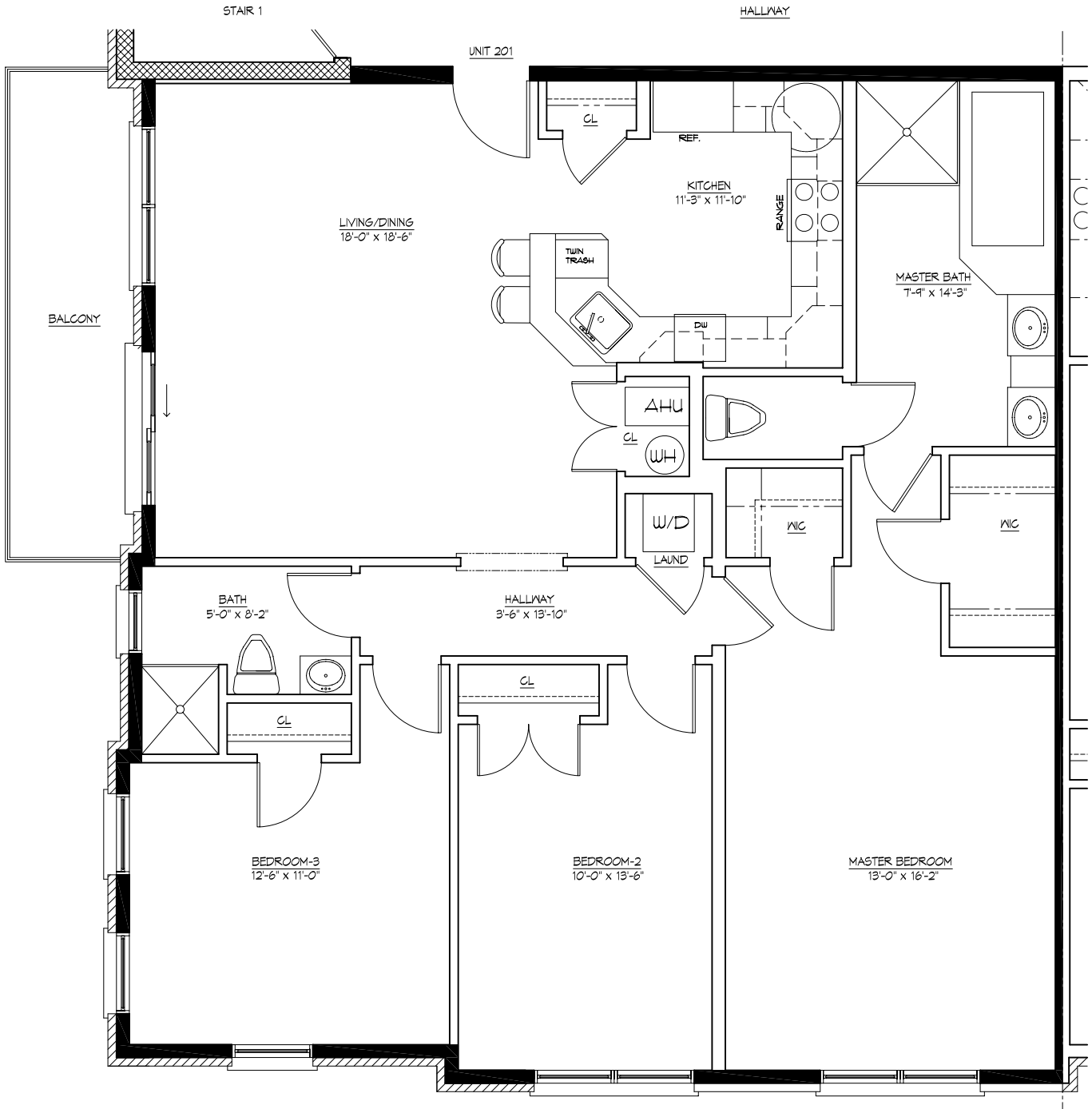
ENLARGED FLOOR PLAN UNIT D UNIT 201, 211, 301, 311 SCALE: NTS
