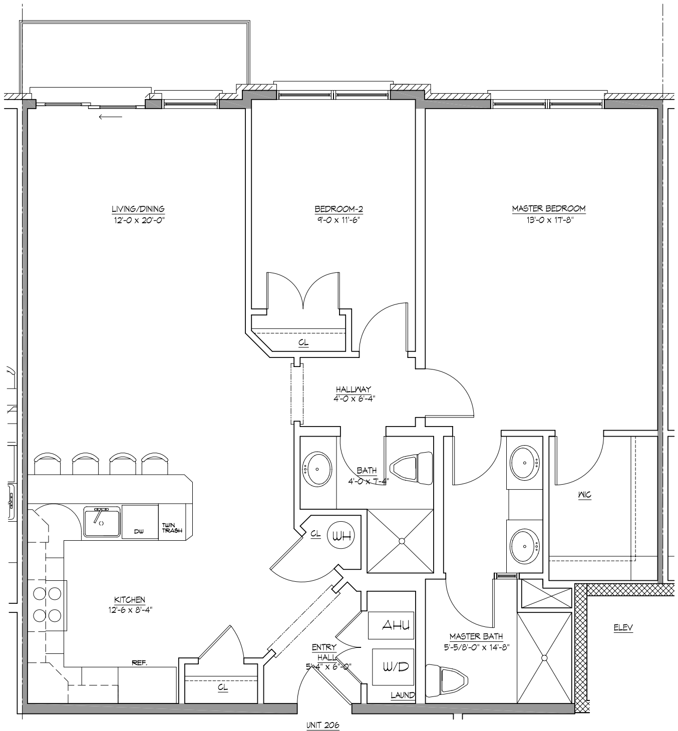
ENLARGED FLOOR PLAN UNIT C UNIT 206, 208 SCALE: NTS
